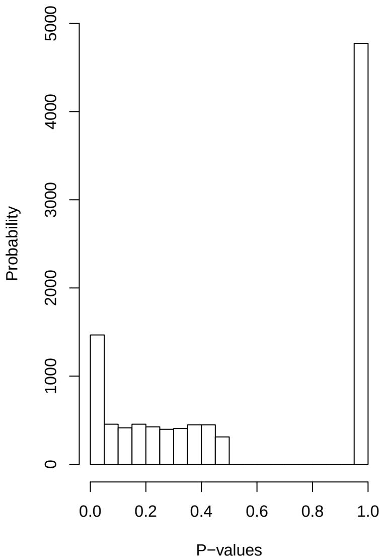
Histogram of P-values
